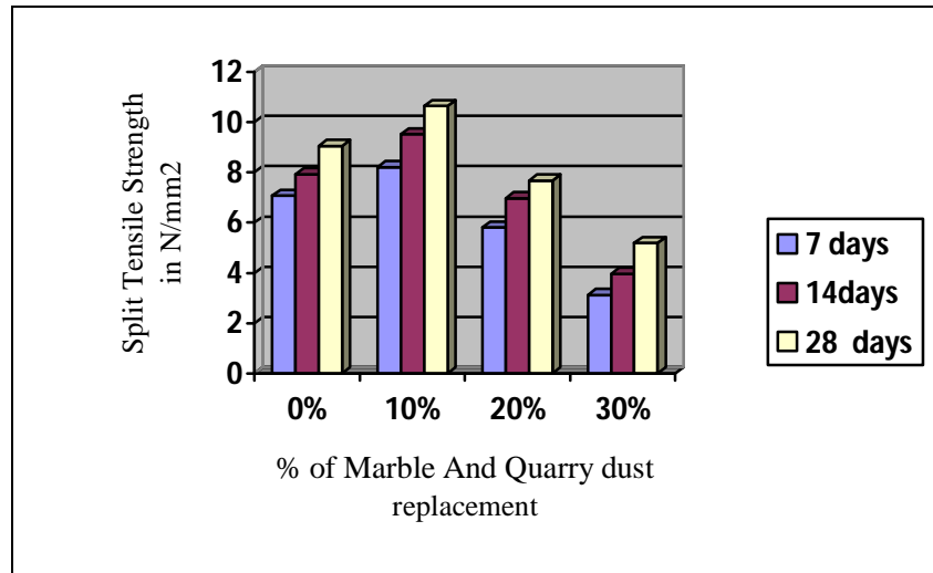
Fig. 2: % replacement of Marble Powder & Quarry Dust vs Split Tensile strength (N/mm 2 )
