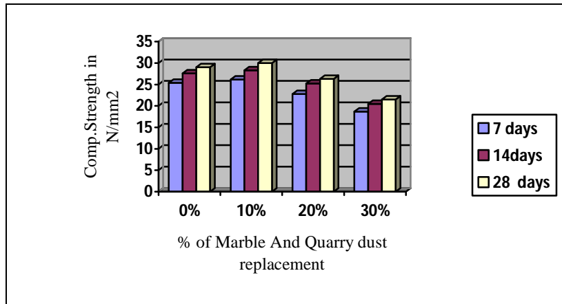
Fig. 1: % replacement of Marble Powder & Quarry Dust vs Compressive strength (N/mm 2 )
