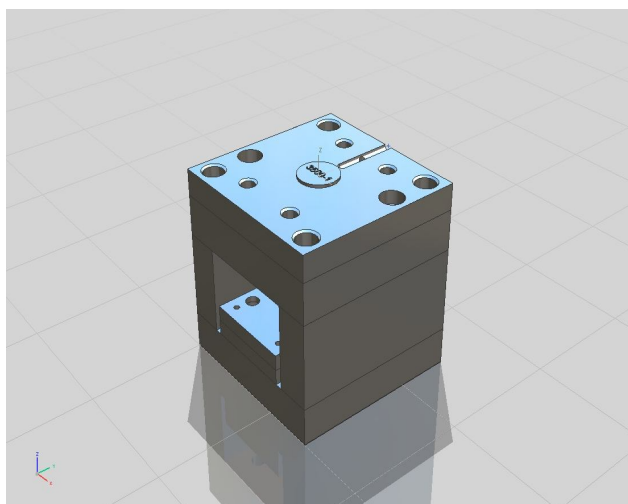
Fig.4. Optimized Mold Structure
