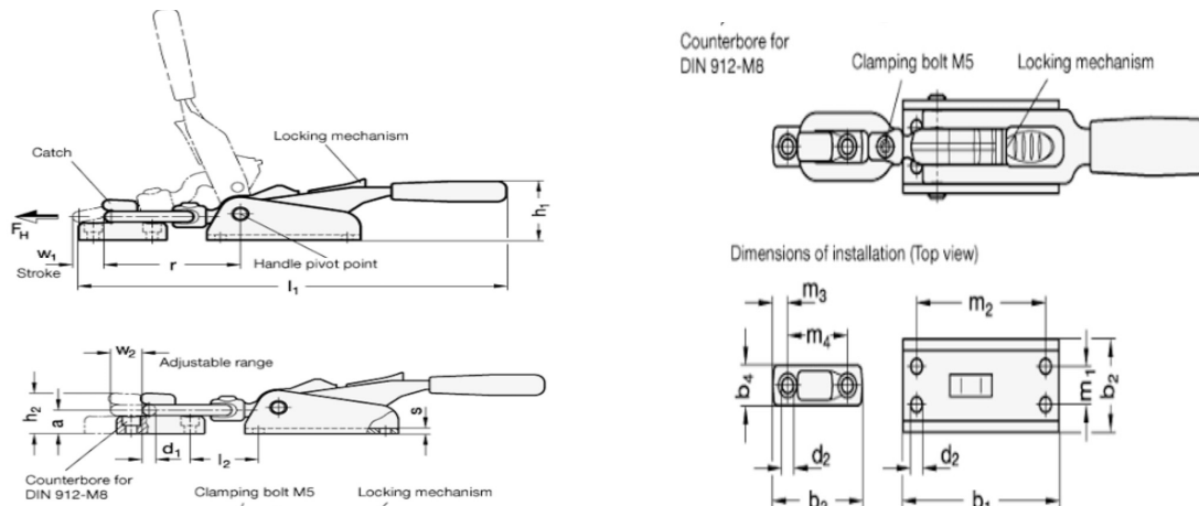
Fig. 2 Latch mechanisms
