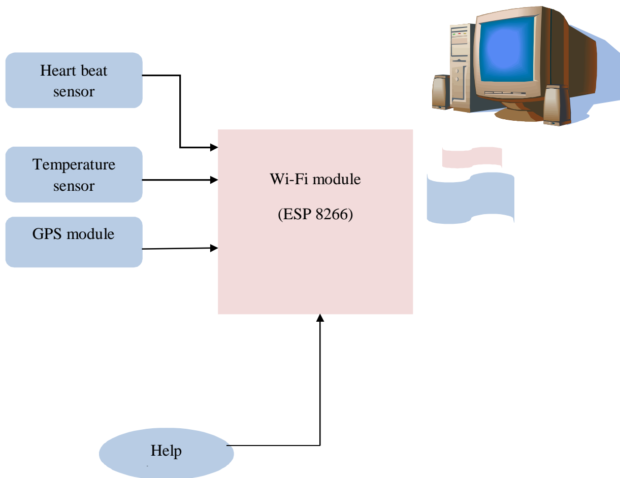
Fig(5.1): Block diagram of soldier unit
