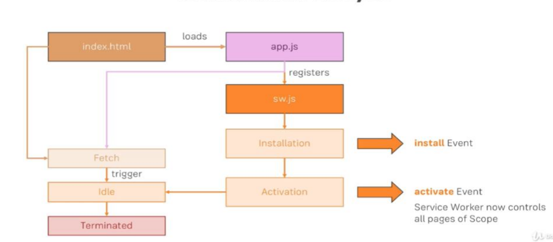
Fig. 2 Service Worker Lifecycle
