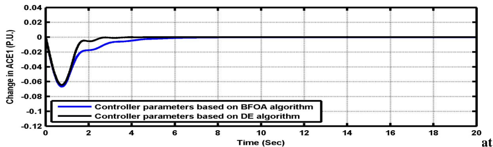
Fig. 15: Tie Line Power Deviation for 5% step change in area-1 with 50% Increase in T_g at \alpha=0.05
