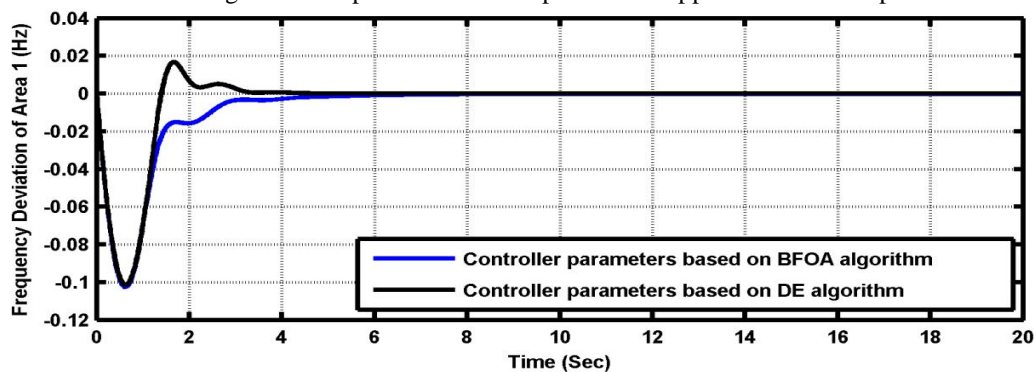
Fig. 7: Frequency Deviation of Area-1 for 5% Step Load Change in Area-1 at \alpha=\pm 0.05
