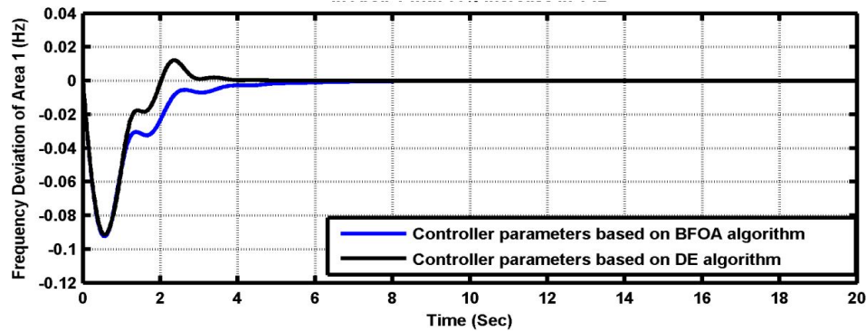
Fig. 13: Frequency Deviation of Area-1 for 5% step change in area-1 with 50% Increase in T_{12} at \alpha=0.05
