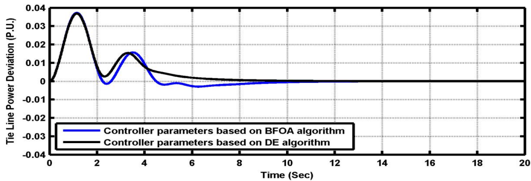
Fig. 12: Tie Line Power Deviation for 5% Step Load Change in Area-2 at \alpha=0.025
