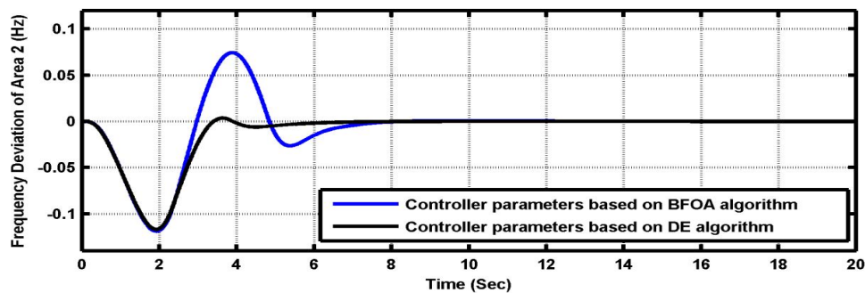
Fig. 14: Frequency Deviation of Area-2 for 5% step change in area-1 with 50% Decrease in T_{12} at \alpha=0.025
