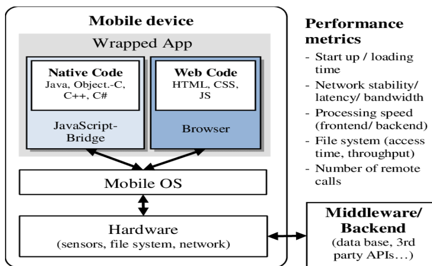
Figure 1: Structure of Hybrid Mobile Application
