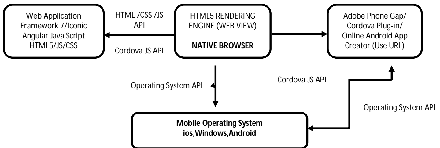
Figure 2 : Novel Framework for Hybrid Mobile Application Development
