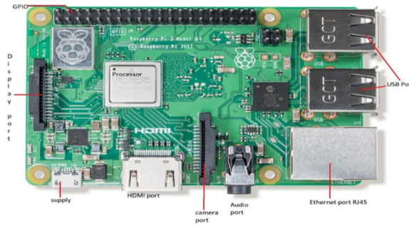
Fig.6. Raspberry Pi
