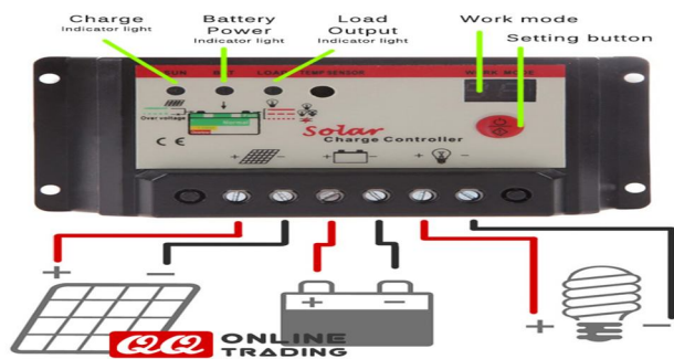
Fig.4.4 Charge Controller
