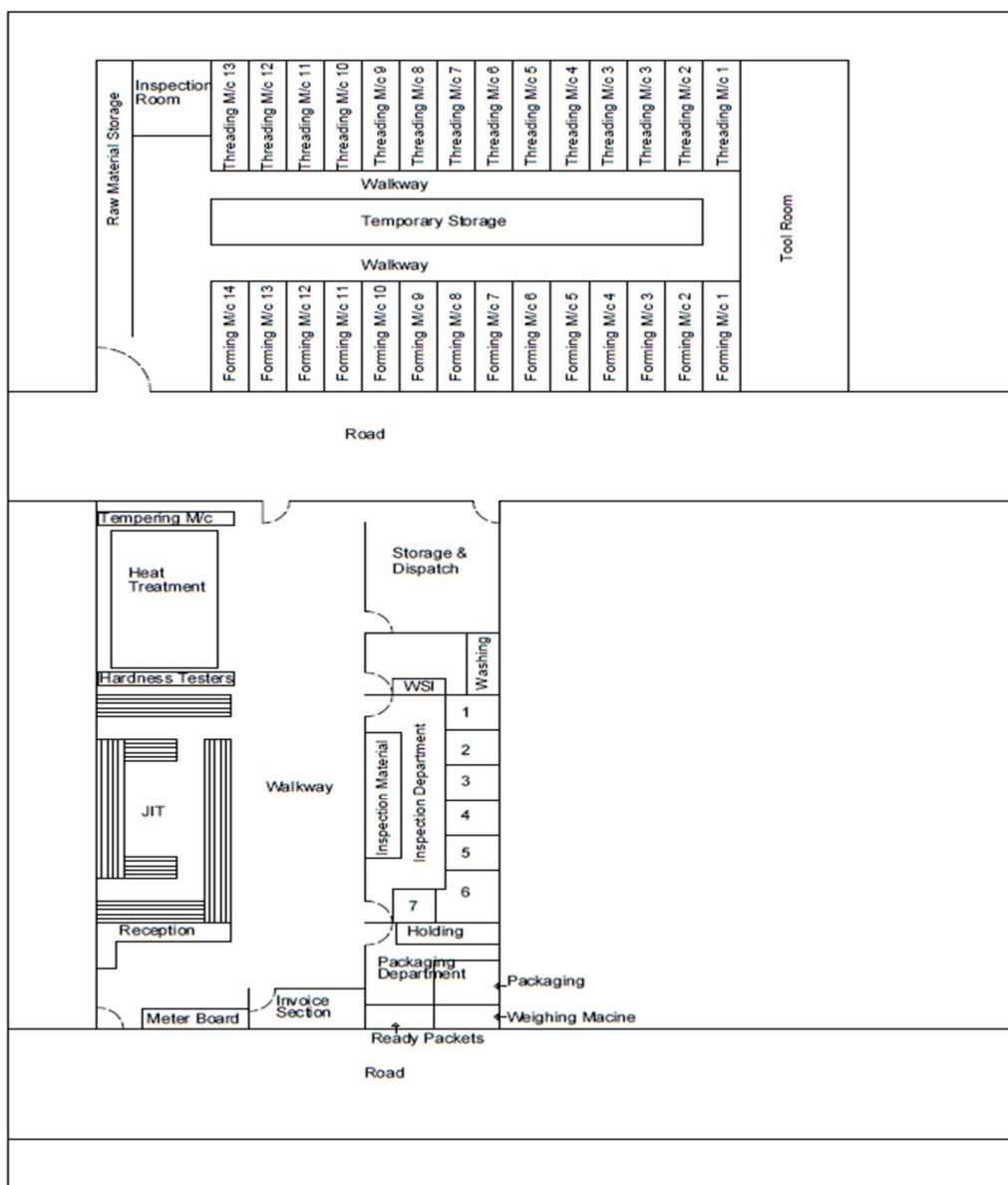
Figure 3.1 Existing plant layout [1]
