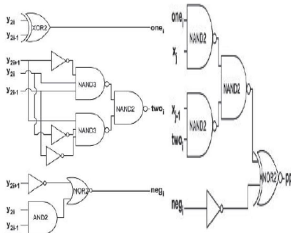
Fig.4: MBE signal generation [10] Fig.5: Partial Product Generation [10]
