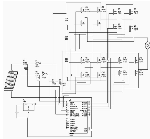
Fig.1. Circuit Diagram
