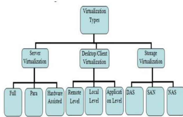
Fig. 8 Virtualization types
