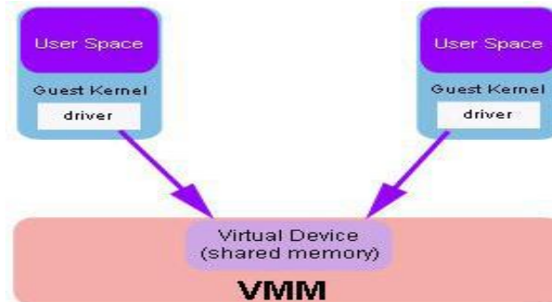
Fig. 7 ZIVM Architecture
