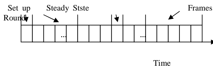
Fig.1 Timeline Showing Operation of LEACH
