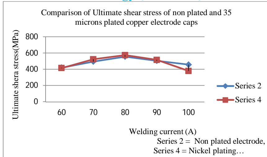
Fig 9: Effect of welding current and 35 microns plating on ultimate shear strength.
