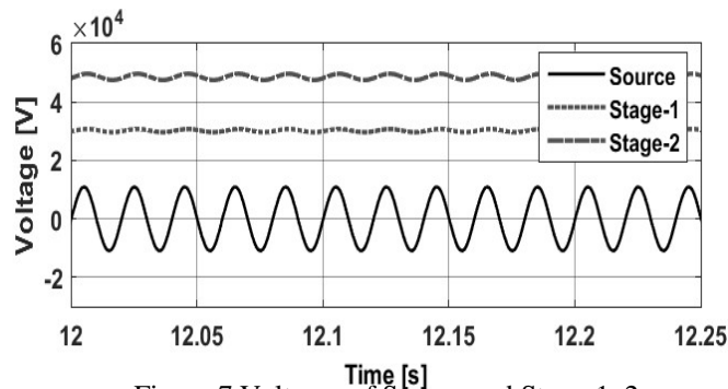
Figure 7 Voltages of Source and Stage-1, 2
