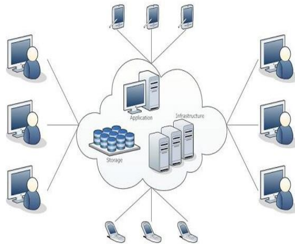
Figure 1: Cloud Computing
