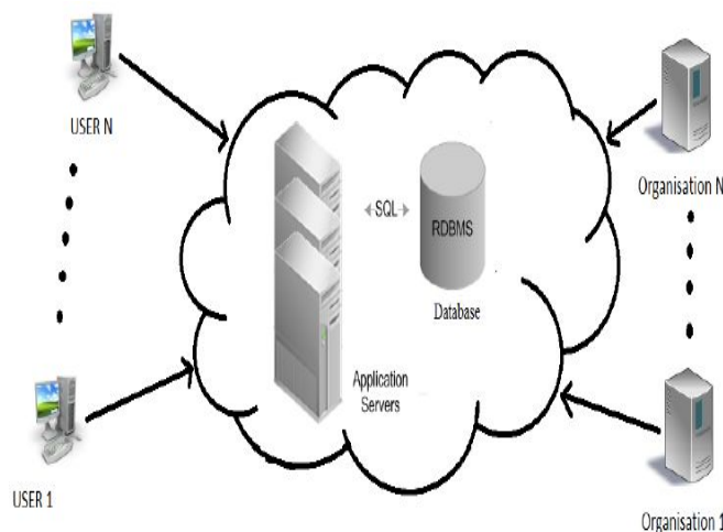
Figure 1: Cloud Computing [11]
