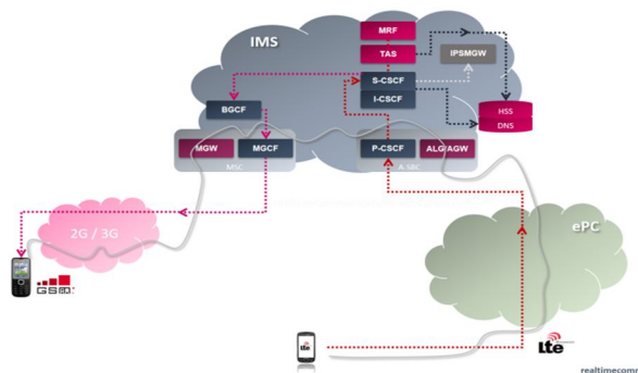
Fig 2. VoLTE Architecture
