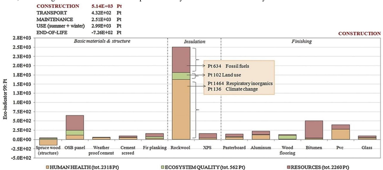
Fig. 5 Life cycle phases of a passive house for 75 years and results from the construction phase to year 0 according to the Eco-indicator 99 method [57]
