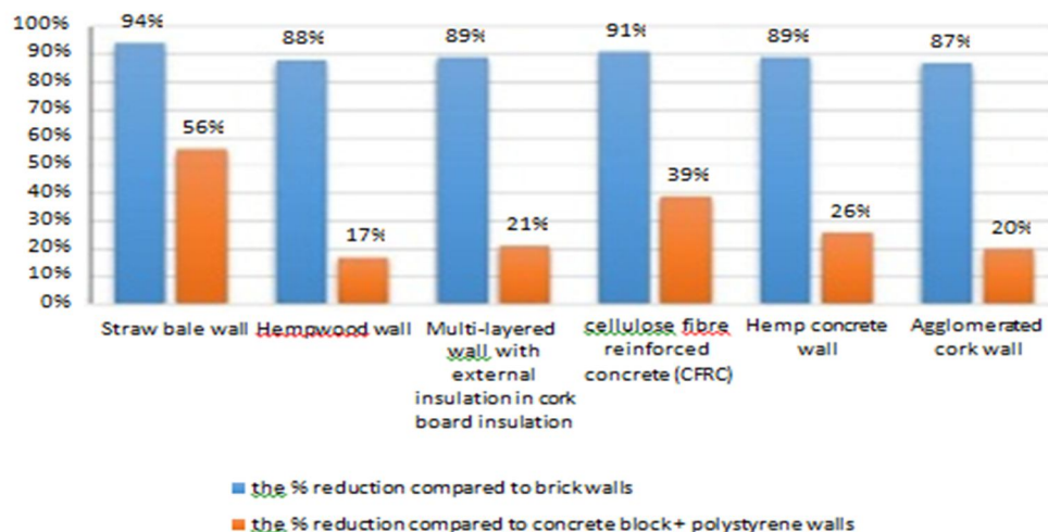
Fig. 23 Percentage reduction in thermal transmittance compared to conventional walls
