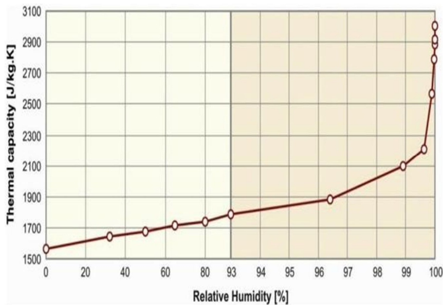
Fig. 21 The Relationship between hemp concrete’s relative humidity and thermal capacity [126]
