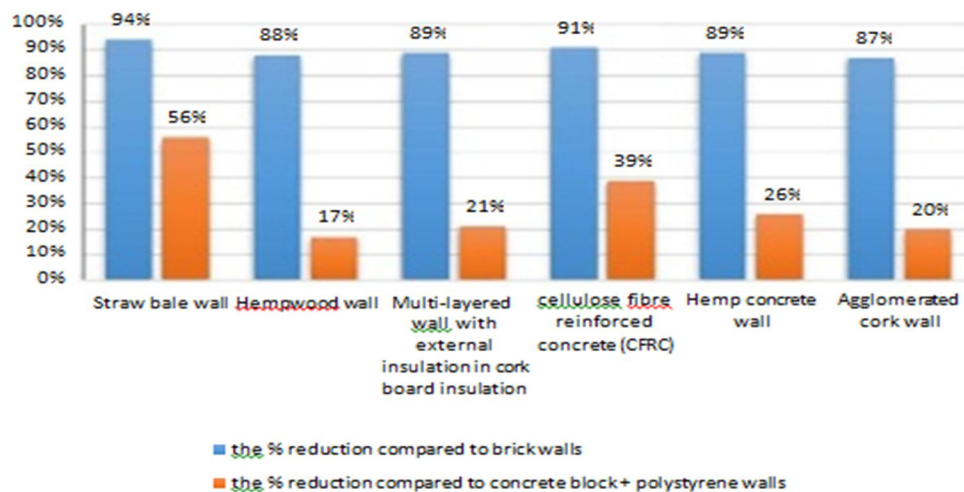
Fig. 23 Percentage reduction in thermal transmittance compared to conventional walls
