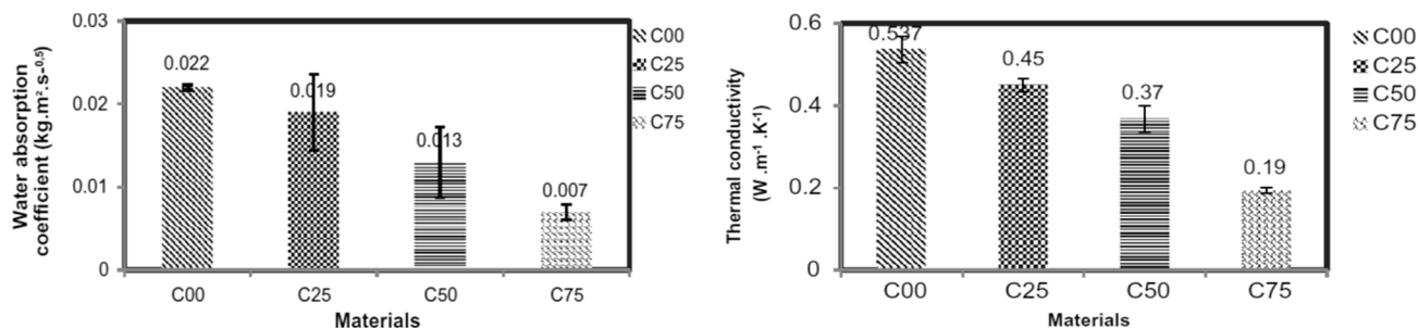
Fig. 17 The standard deviation of the absorption coefficient and thermal conductivity of cork cement composites [122]
