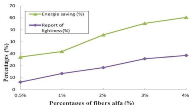
Fig. 12 Energy savings and lightness ratio evolution as a function of Alfa fibre percentages [92]
