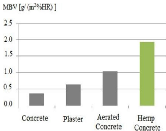
Fig. 22 moisture buffer value (WBV) of common materials and hemp concrete[157]
