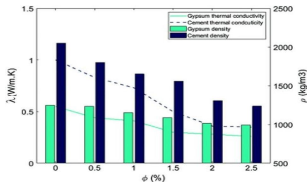
Fig. 8 The composite's thermal conductivity and density as a function of the fibre ratio [73]
