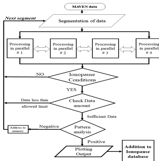
Figure 5.1: The Flowchart explaining Data processing by YAILDA
