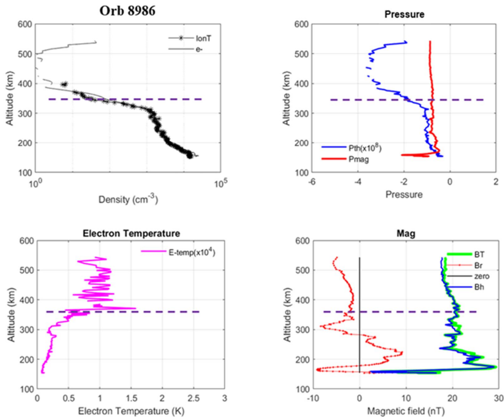
Fig. 5.2 Orbit 8986 Altitude profiles of the (a) Total ion and Electron density (b) Magnetic and Thermal pressure (c) Electron Temperature and (d) Magnetic field components. The ionopause is marked with dashed line.
