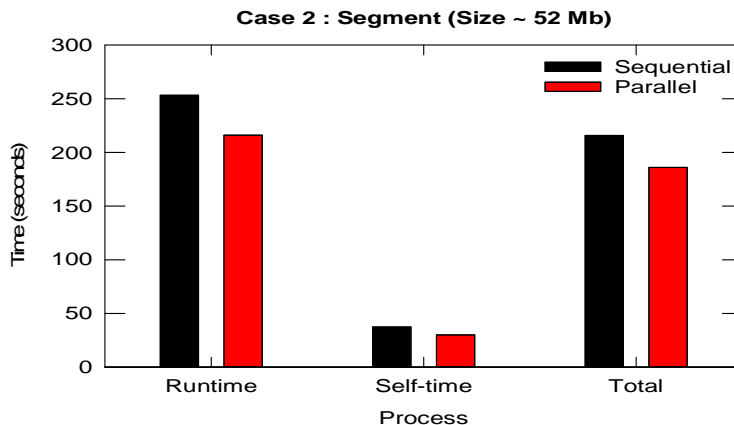
Fig. 6.2 Time taken to process Segment in sequential (black colour) and parallel (red)
