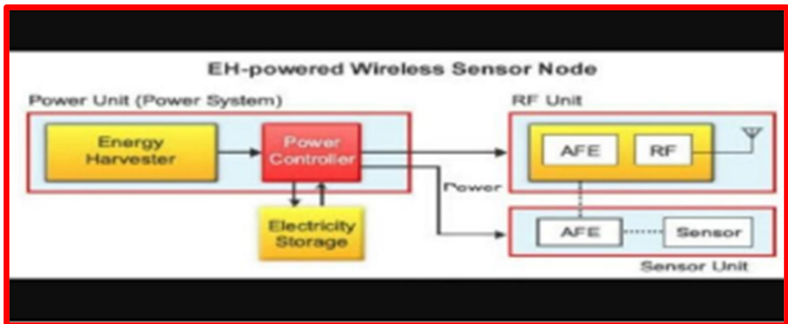
Fig.14: Wireless Sensors
