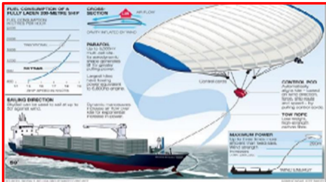
Fig.8: Wind /kite-power cargo ships.
