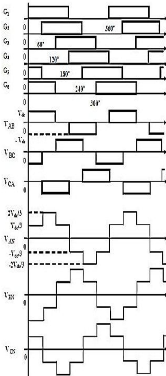
Fig: 4 Conduction of inverter
