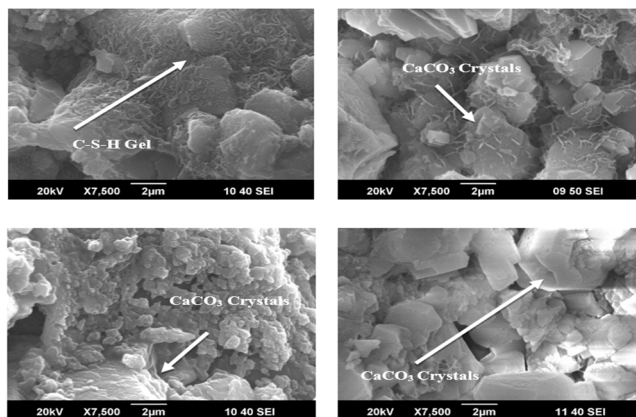
Figure 7: 7 days bacterial concrete effects on SEM
