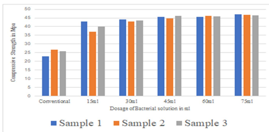
Figure 4: Compressive Strength graph for 14 days
