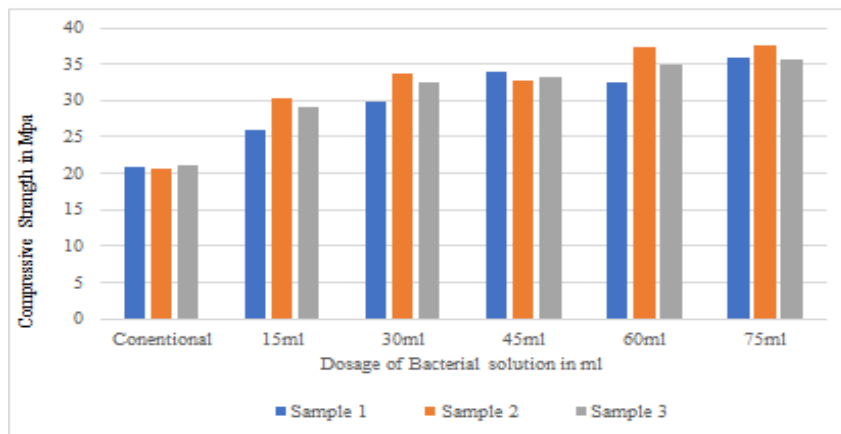
Figure 3: Compressive Strength Graph for 7 Days
