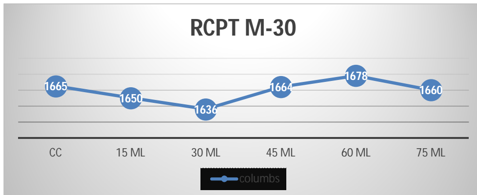
Figure 6: RCPT coulombs
