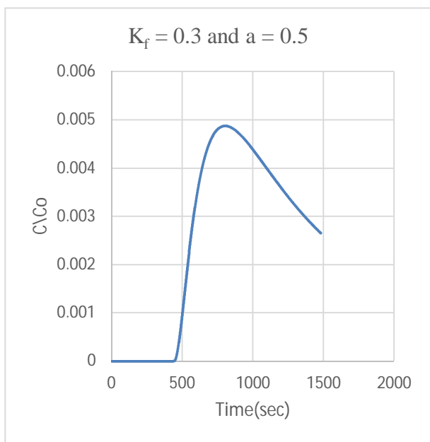
Figure 13: Breakthrough curve for a = 0.5 and K_f = 0.3
