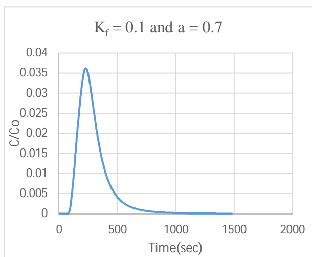
Figure 2: Breakthrough curve for a = 0.7 and K_f = 0.1
