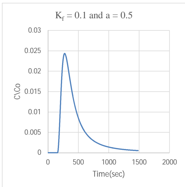
Figure 11: Breakthrough curve for a = 0.5 and K_f = 0.1
