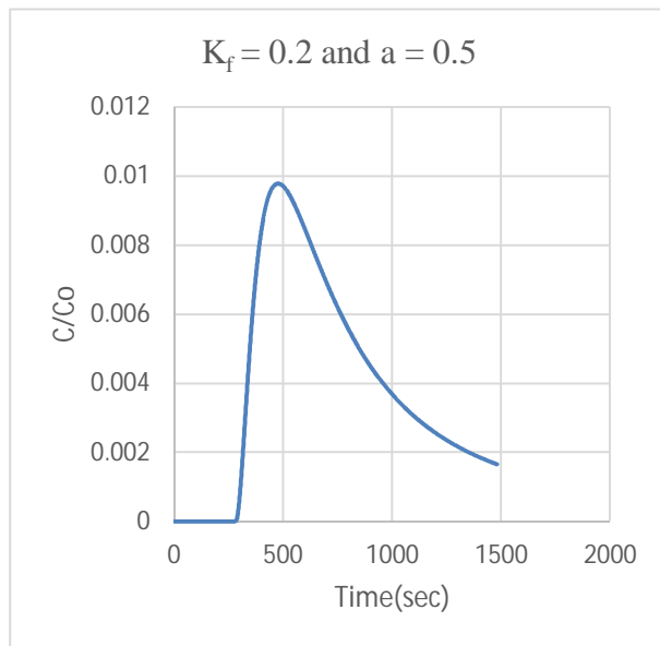
Figure 12: Breakthrough curve for a = 0.5 and K_f = 0.2
