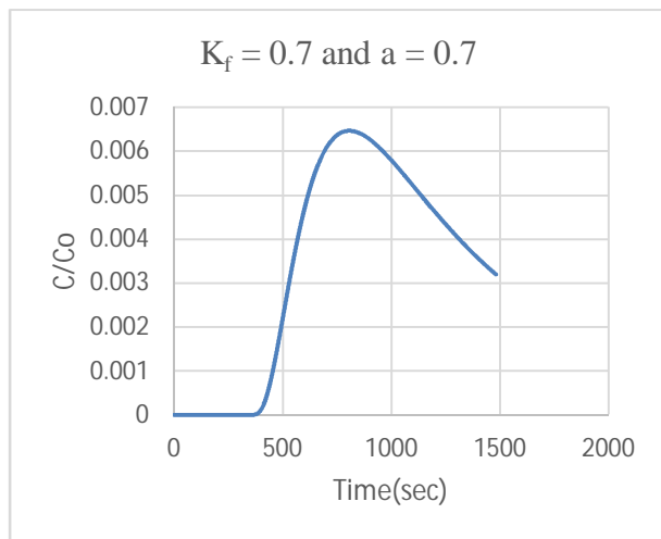
Figure 8: Breakthrough curve for a = 0.7 and K_f = 0.7
