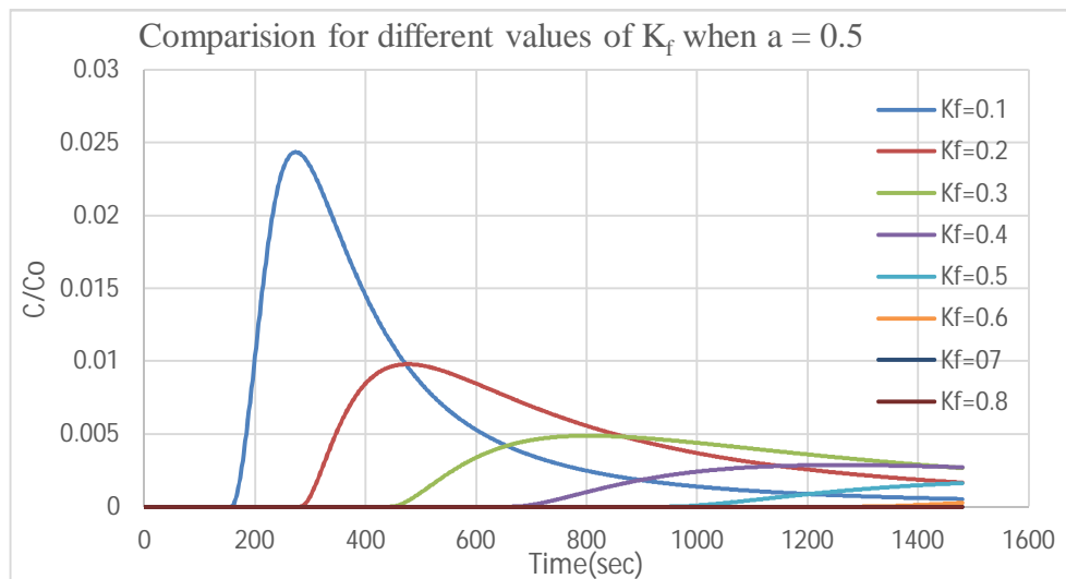
Figure 19: Comparison between different values of K_f when a = 0.50 at 8 cm from source of contaminant.
