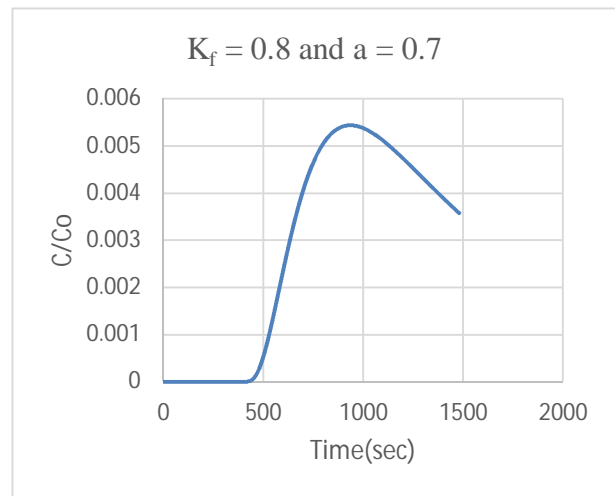
Figure 9: Breakthrough curve for a = 0.7 and K_f = 0.8
