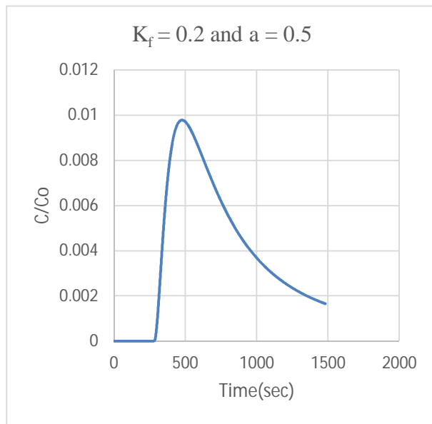
Figure 12: Breakthrough curve for a = 0.5 and K_f = 0.2
