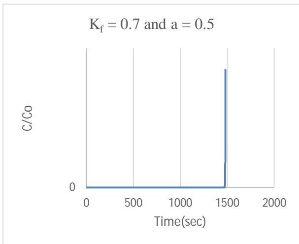
Figure 17: Breakthrough curve for a = 0.5 and K_f = 0.7
