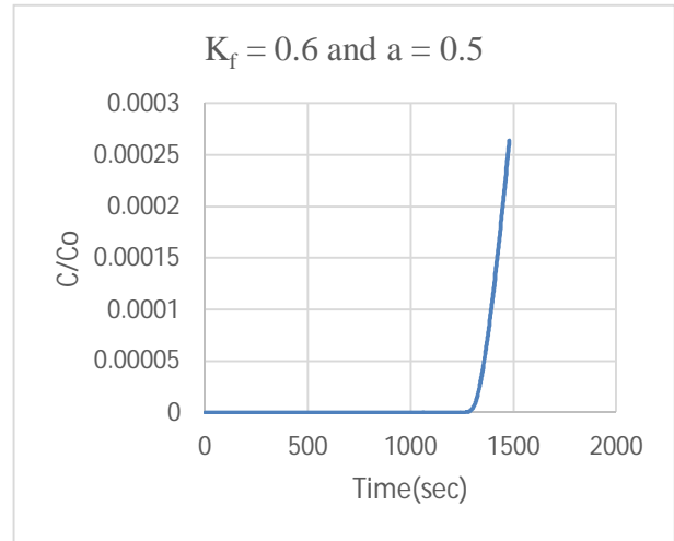
Figure 16: Breakthrough curve for a = 0.5 and K_f = 0.6
