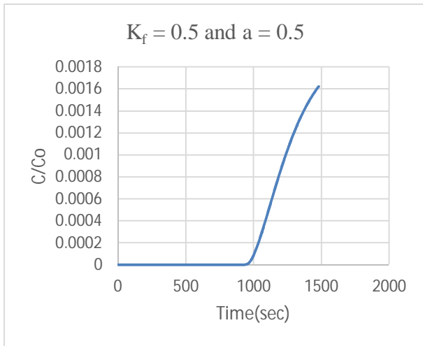
Figure 15: Breakthrough curve for a = 0.5 and K_f = 0.5
