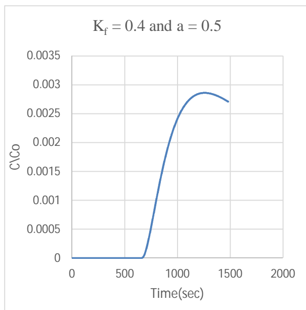
Figure 14: Breakthrough curve for a = 0.5 and K_f = 0.4
