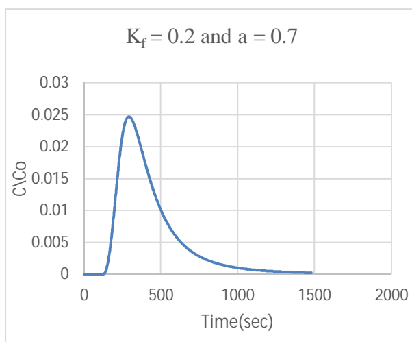
Figure 3: Breakthrough curve for a = 0.7 and K_f = 0.2
