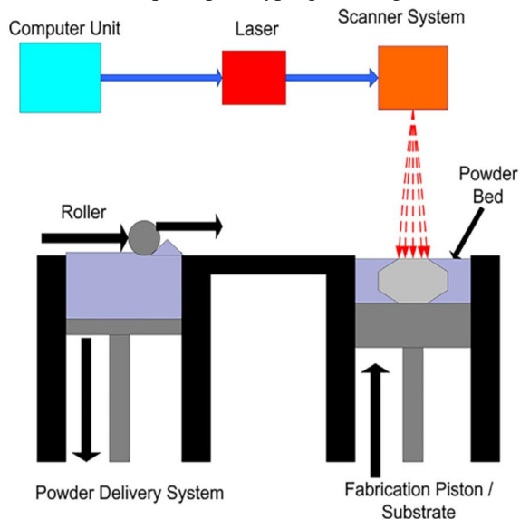
Figure 4: Schematic illustration diagram of direct metal laser sintering method. [16]
