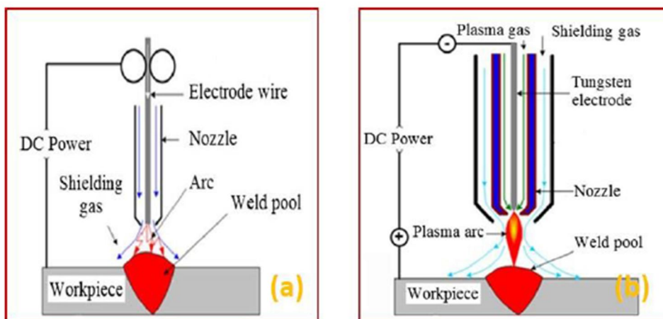
Figure 3: Schematic diagram of MIG Welding, and (b) Plasma Arc Welding Process [14].
