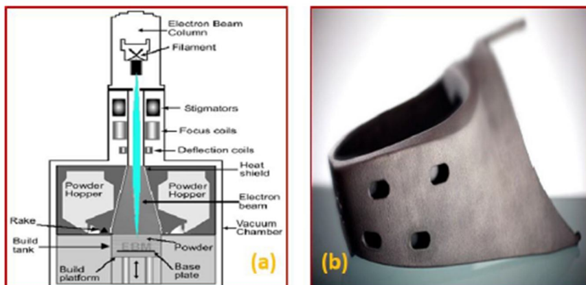
Figure 2: (a) Schematic illustration of AM electron beam melting technique, and (b) fabricated part of aviation. [7]
