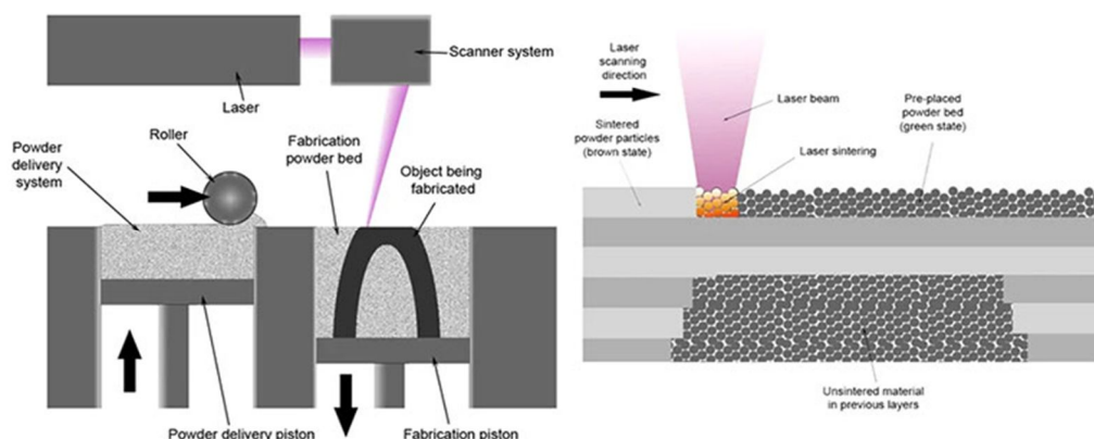
Figure 1: Schematic diagram of SLM 3D printing works. [5]
