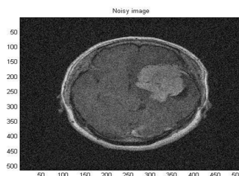
Fig.3.Noisy image
