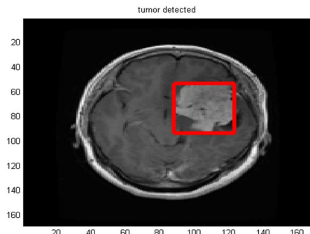
Fig.7.SVMclassification
