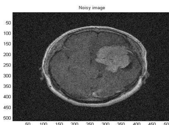
Fig.3.Noisy image
