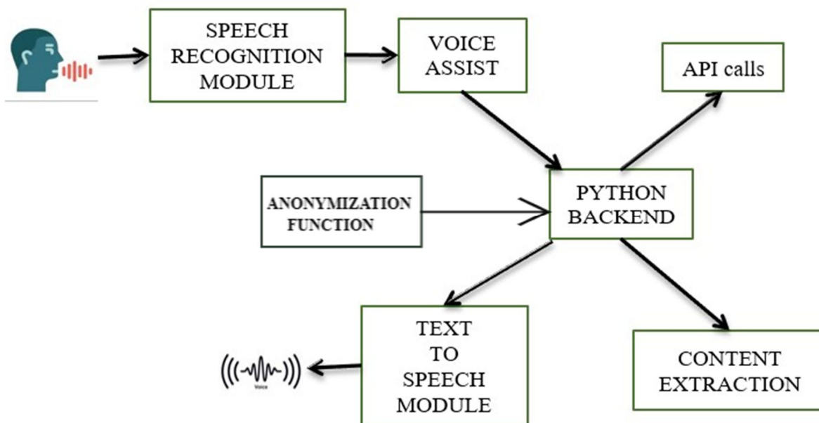
Fig 2 : Workflow model
