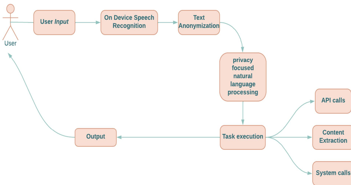
Fig 3 : System Architecture
