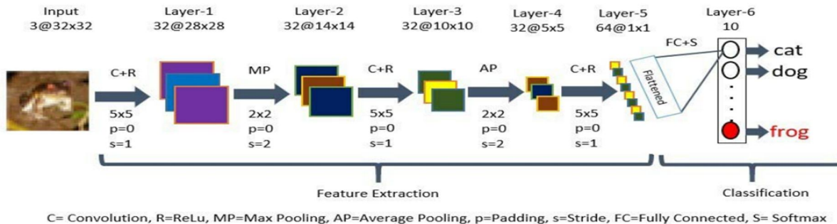
Fig 4. The architecture of our proposed CNN
