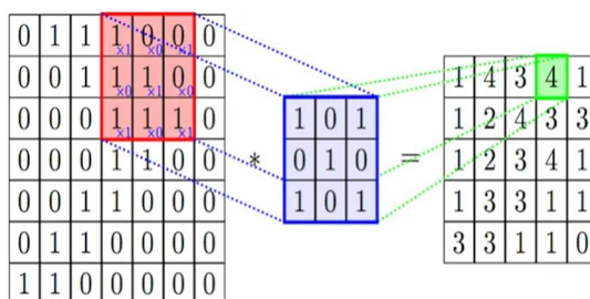
Fig 1. Convolution Operation
