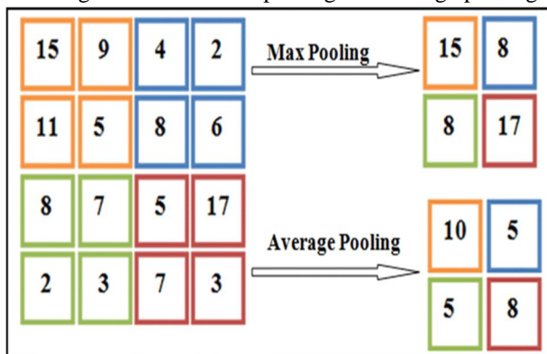
Fig 2. Max pooling and Average pooling operation
