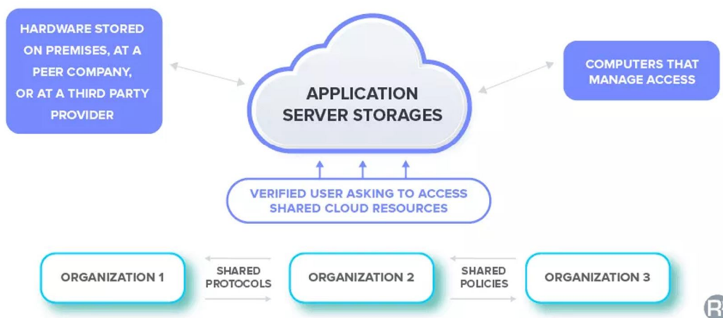
FIG V: COMMUNITY CLOUD
