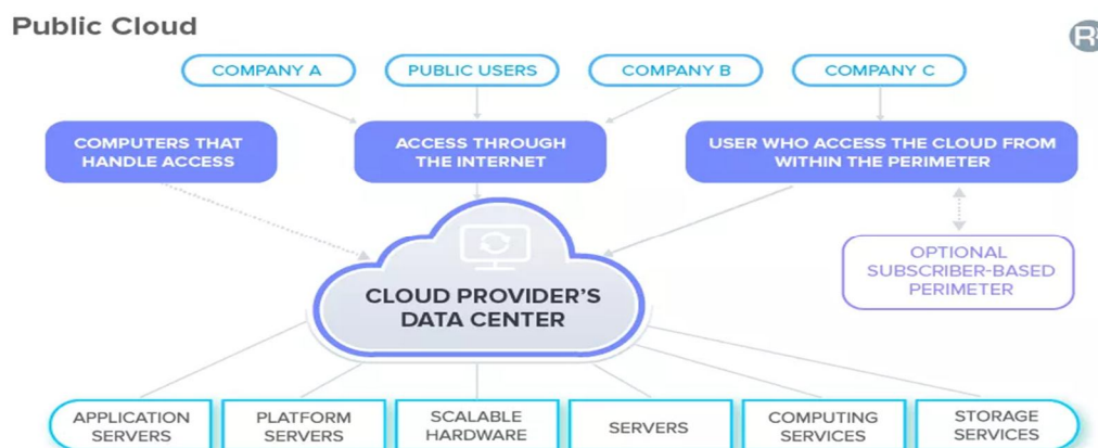
FIG II: PUBLIC CLOUD
