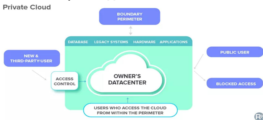
FIG III: Private Cloud
