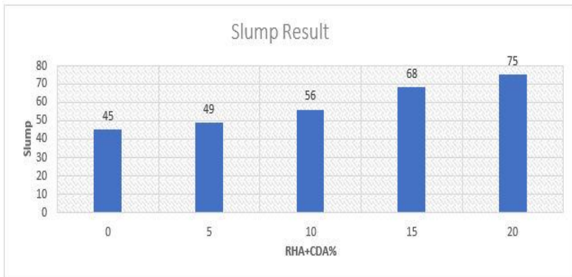
Fig. 6: Slump values for various RHA+CDA% mix
