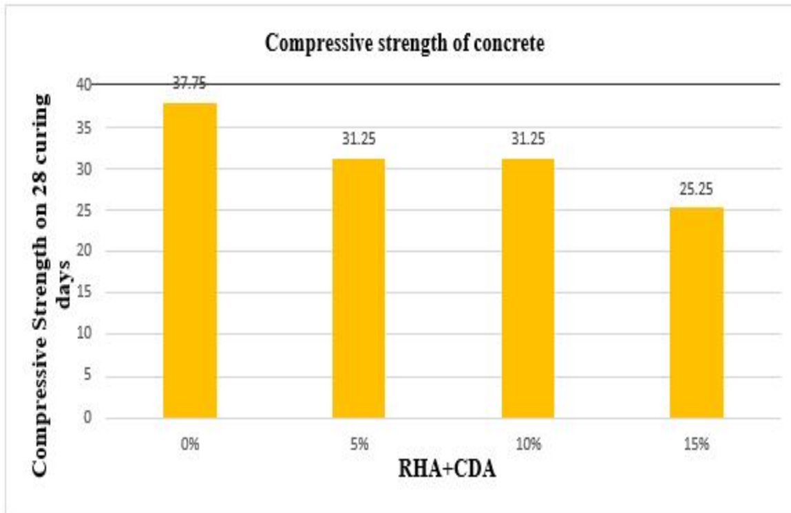
Fig. 8: Compressive strength results for various RHA+CDA% mix at 28 days curing
