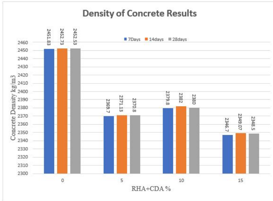
Fig. 7: Density results for various RHA+CDA% mix at 7,14,28 days curing
