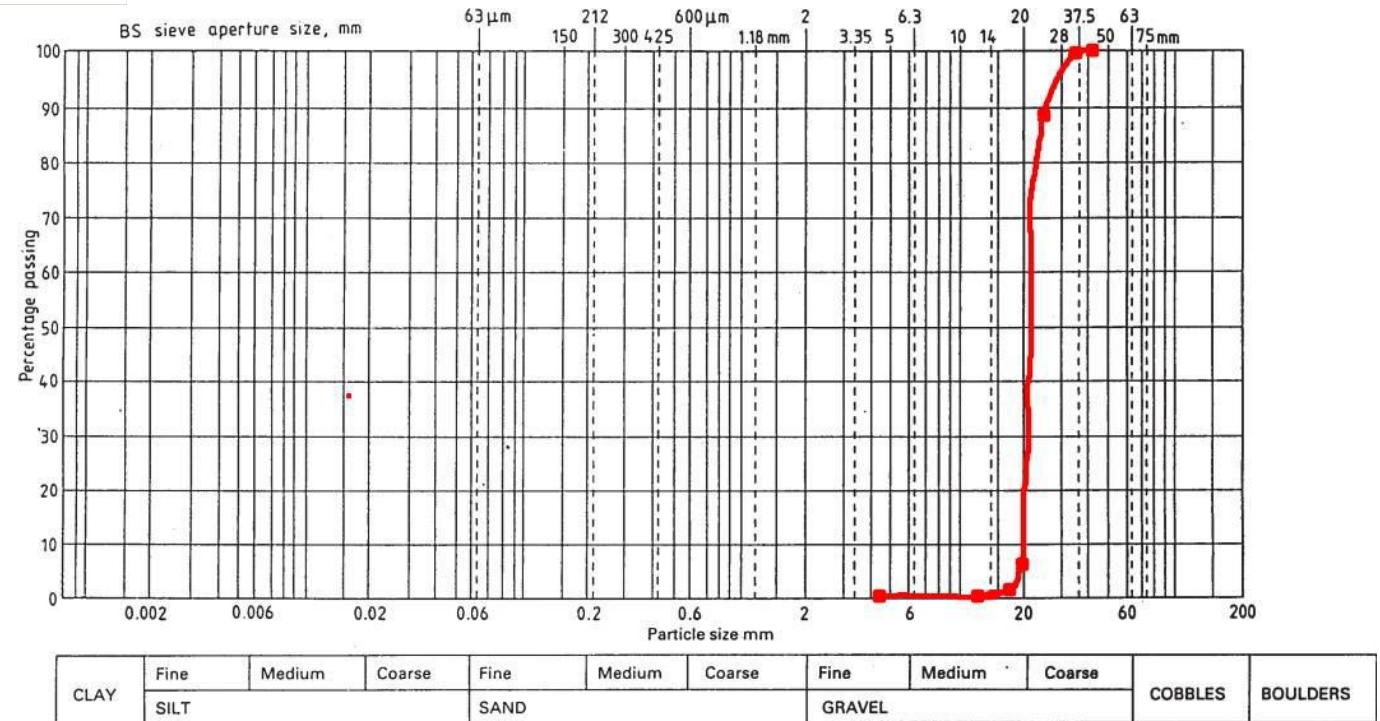
Fig. 5: Gradation Curve for Coarse Aggregate
