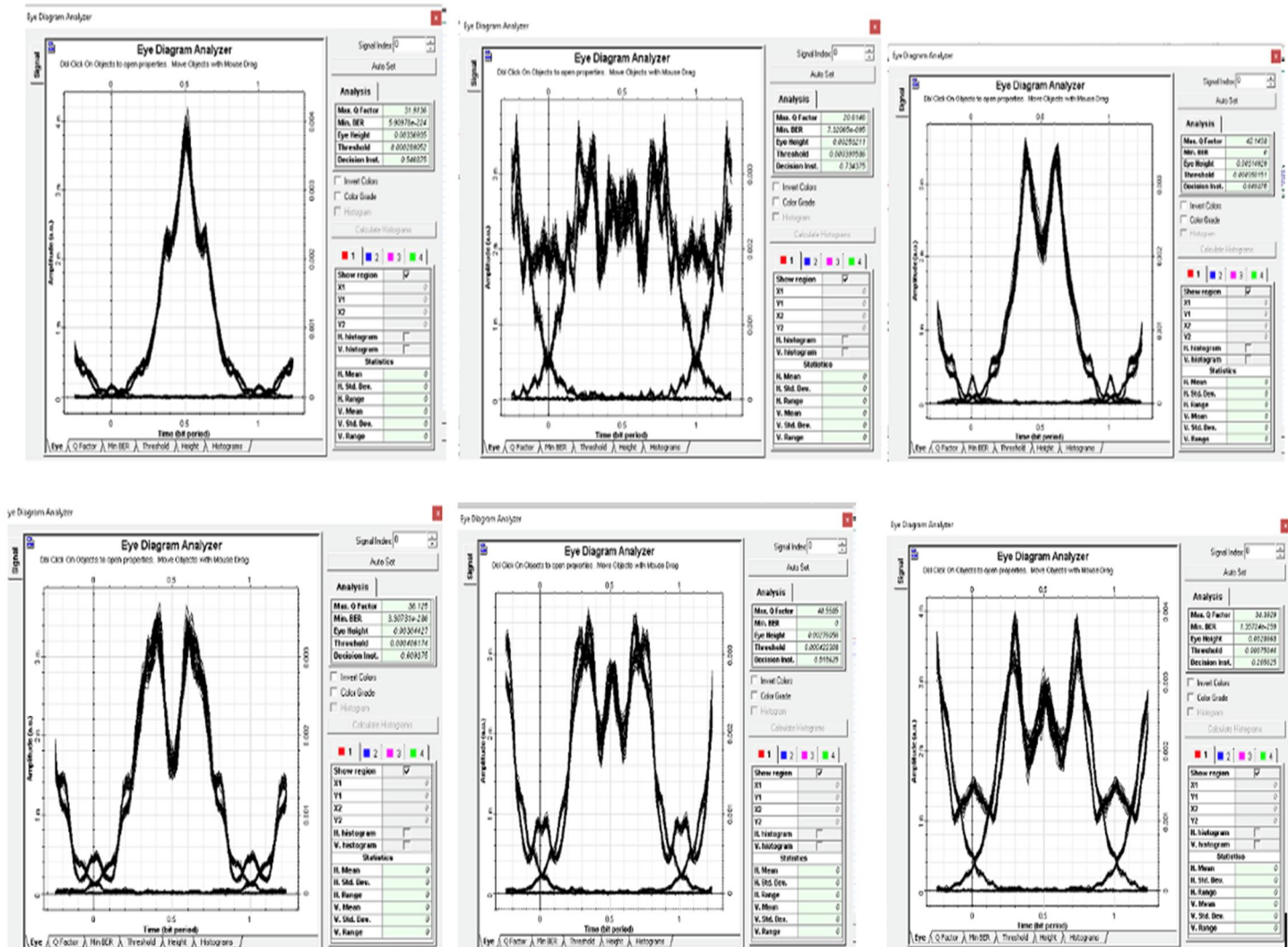
Fig 12: Eye Diagram Results
