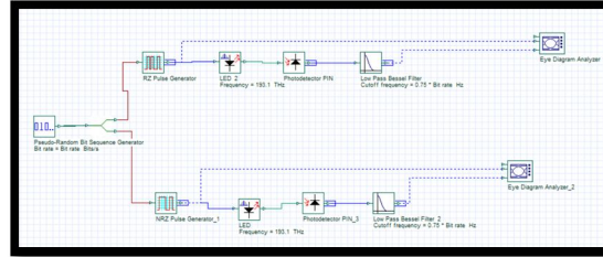
Fig 8: Simulation Setup Setup with no Mach Zehnder Modulator
