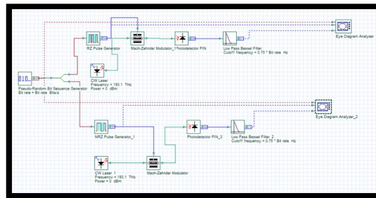
Fig 10: Simulation Setup with Mach Zehnder Modulator
