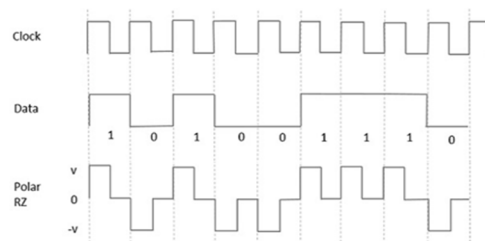
Fig 6: Polar RZ coding
