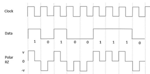
Fig 6: Polar RZ coding
