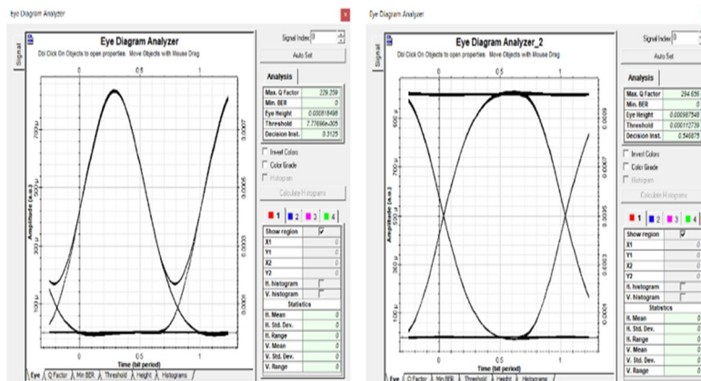
Fig 11: Eye Diagram Results
