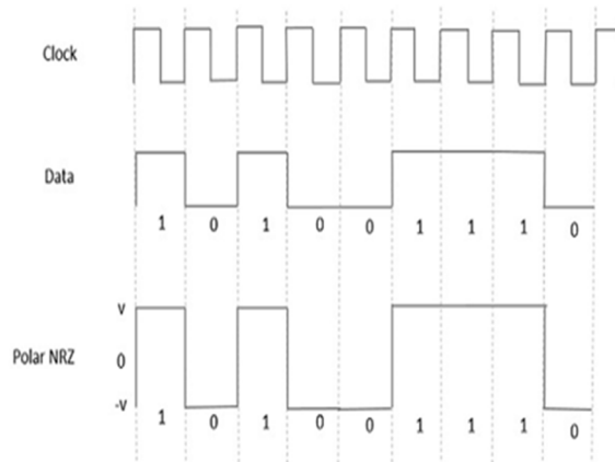
Fig 3: Polar NRZ coding
