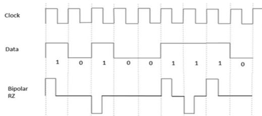
Fig 7: Bipolar RZ coding
