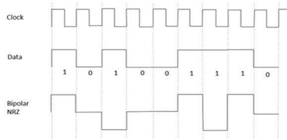
Fig 4: Bipolar NRZ coding
