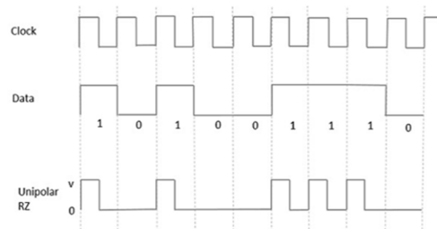
Fig 5: Unipolar RZ coding
