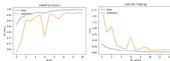
Fig 4: Accuracy and loss curves for ResNet
