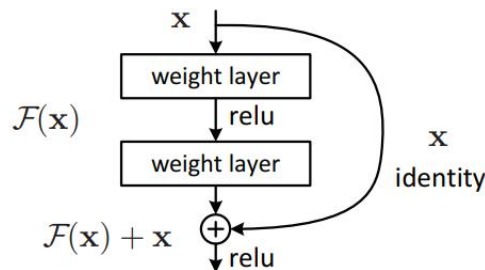
Fig 2: Residual Network Block
