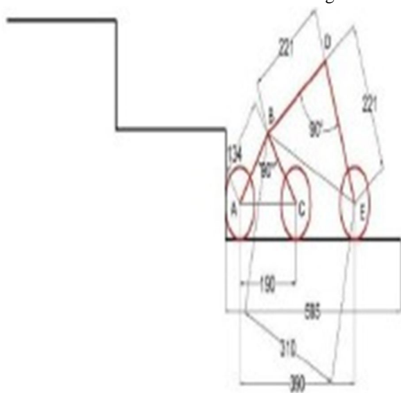
Fig.2. Cad drawing for first triangle
