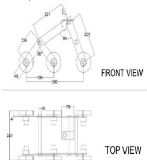
Fig.5.2 Drawing of Rocker Bogie Mechanism
