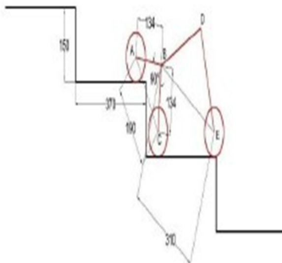
Fig 3 Cad drawing for second triangle
