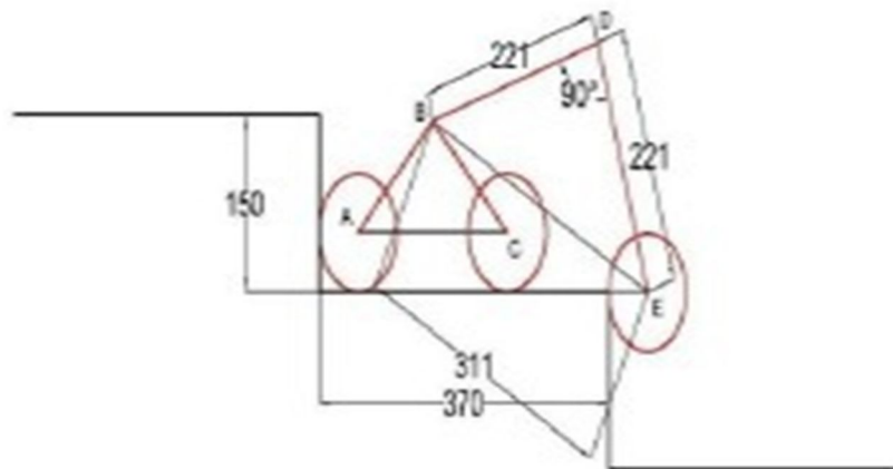
Fig.4. CAD drawing of both triangles
