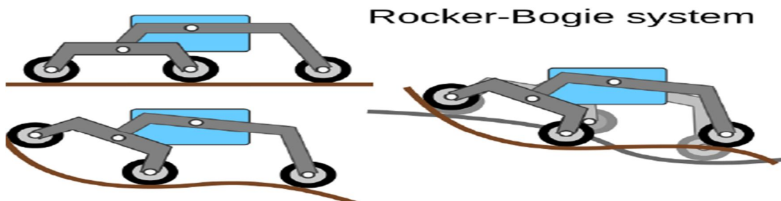
Fig.1: Mechanism of rocker-bogie suspension
