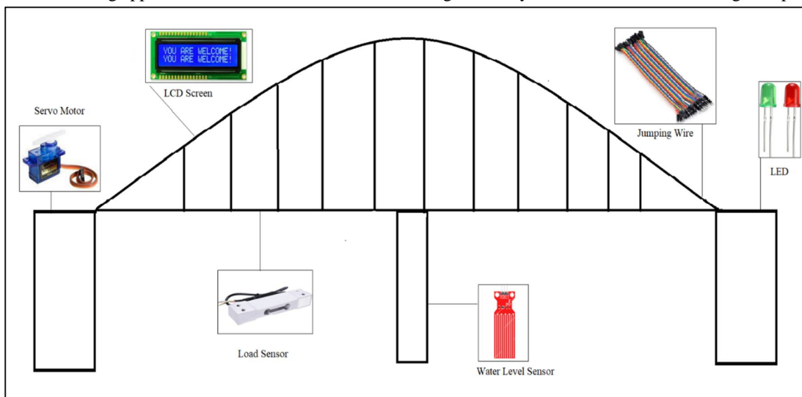
Fig.1 Placement of hardware components on the bridge
