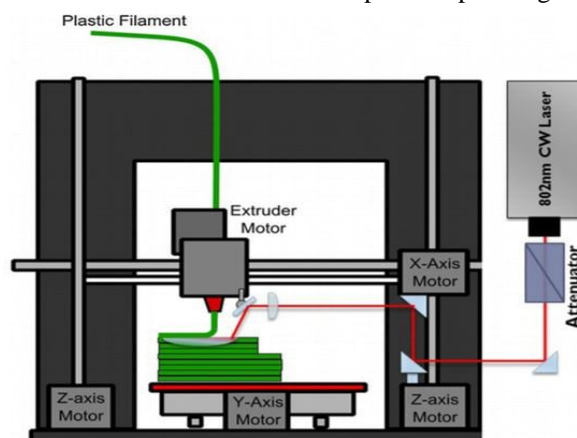
Fig 1. 3d printer operation
