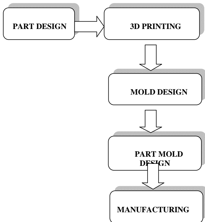
Fig 3. Methodology
