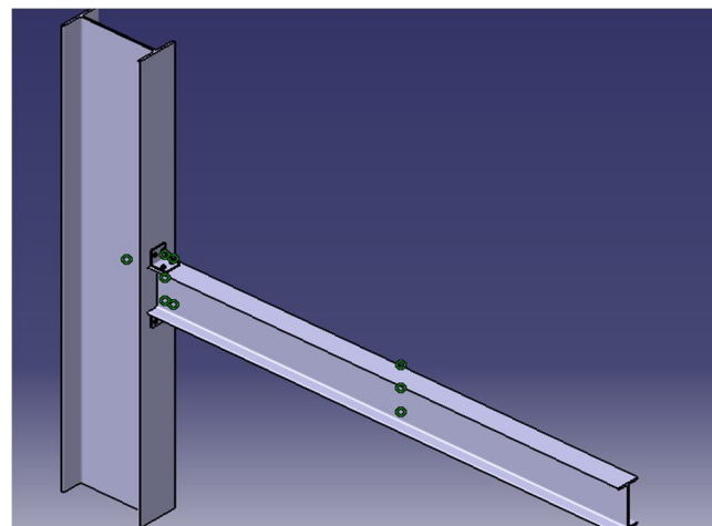
Fig 5 : Top and seat cleats model
