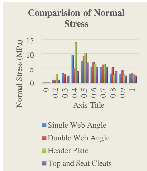
Graph 4: Normal Stress
