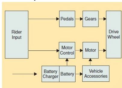
Fig 1. Block Diagram
