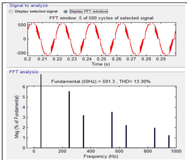
Fig(3)output and THD in harmonics order in phase1 withoutseries compensation
