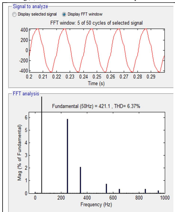
Fig (7)output and THD in harmonics order in phase1 with series compensator
