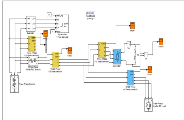
Fig(2)simulink model without series compensation
