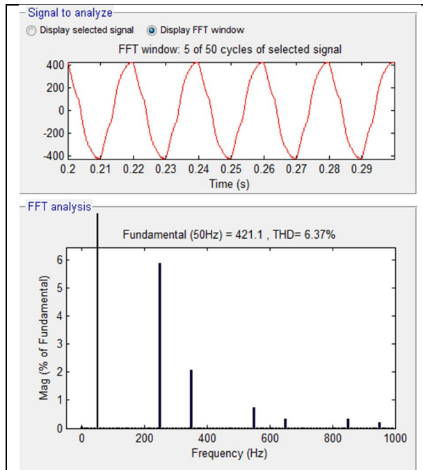
Fig (9) output and thud in harmonics order in phase1 withseries compensator
