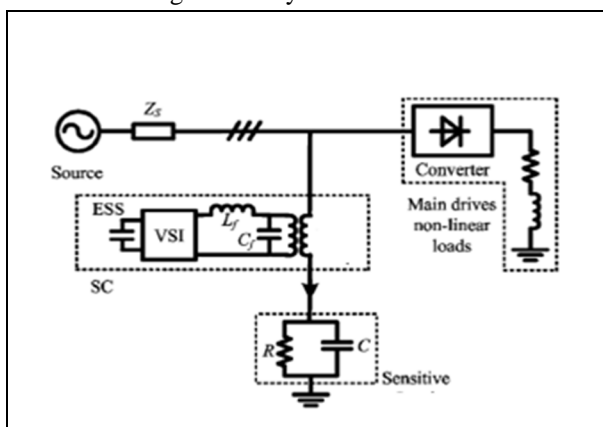
Fig-1 Typical isolated power system model
