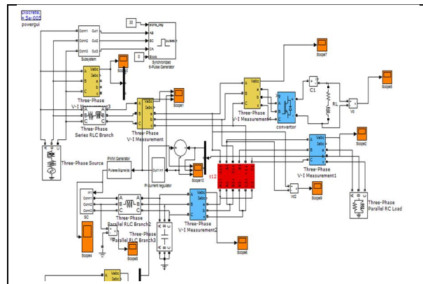
Fig(6)simulink model with series compensation
