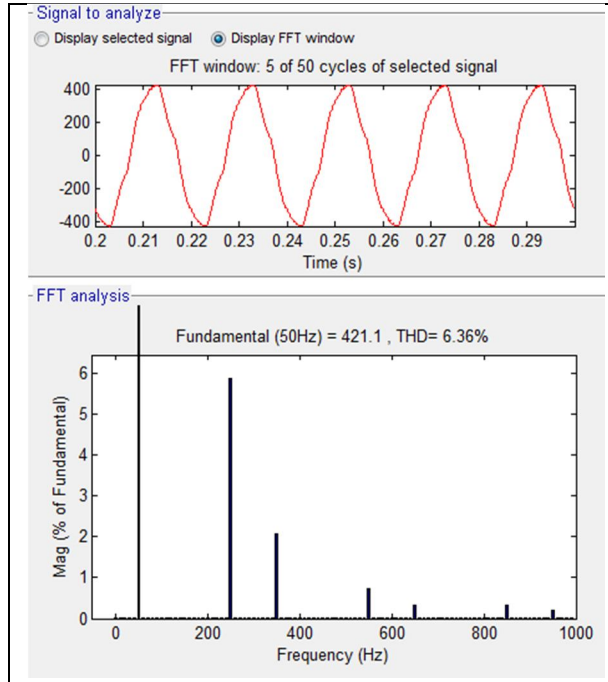
Fig(8)output and THD in harmonics order in phase2 with seriescompensator
