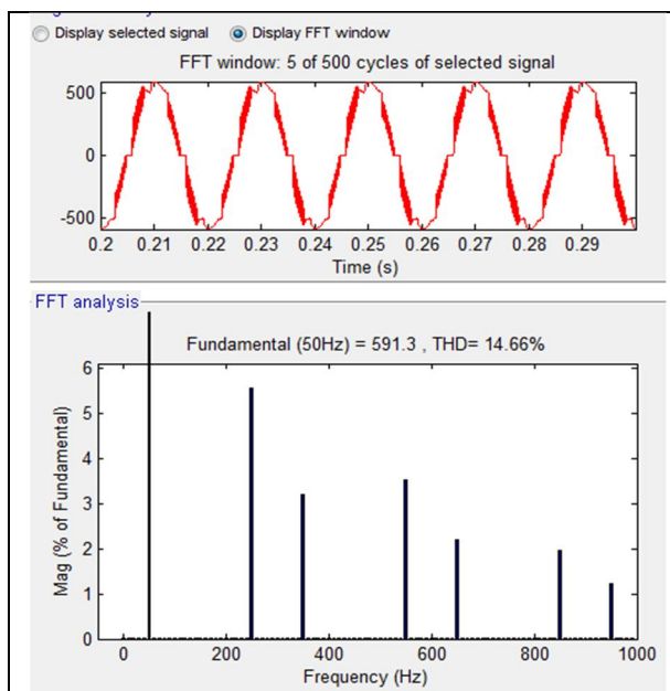
Fig(4)output and THD in harmonics order in phase2 without series compensator
