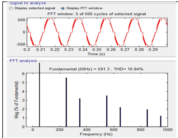
Fig(5) output and THD in harmonics order in phase3 without series compensator
