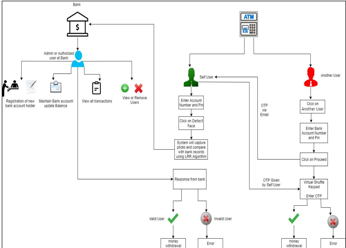
Fig 1: System Architecture
