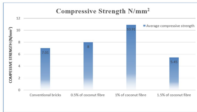
Fig 9 Average Compressive Strength of bricks
