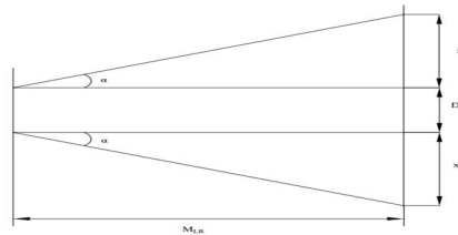
Fig 6. Headlight beam top views geometrical parameters
