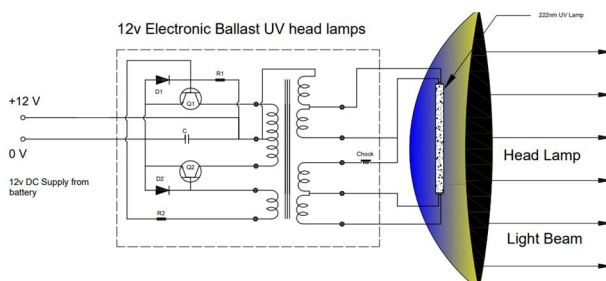
Fig 8. Circuit diagram of 12-V ballast with UV headlamps
