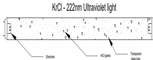
Fig 9. Structural diagram of the KrCl-222 nm UV lamp
