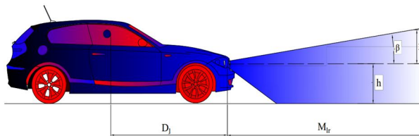
Fig 4. (a) (b)Headlight beam geometrical parameters.
