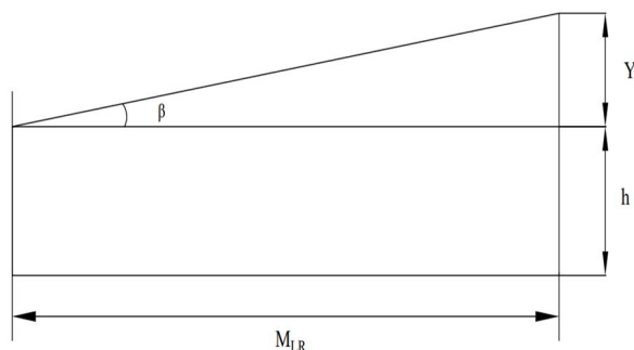
Fig 5. Headlight beam side views geometrical parameters
