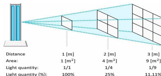
Fig 7. UV-C light propagation based on the inverse square law [25]
