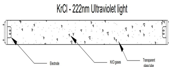
Fig 9. Structural diagram of the KrCl-222 nm UV lamp
