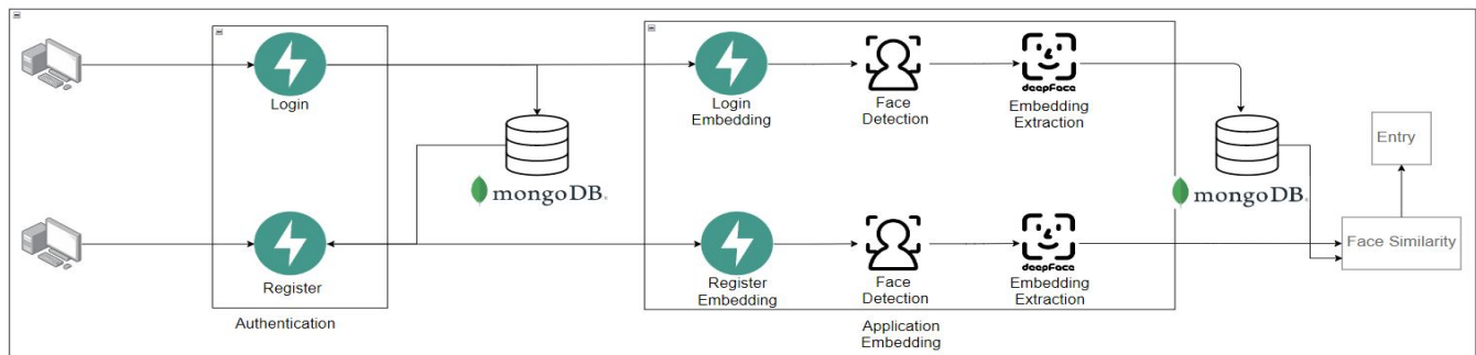
Fig .1. Authentication system workflow
