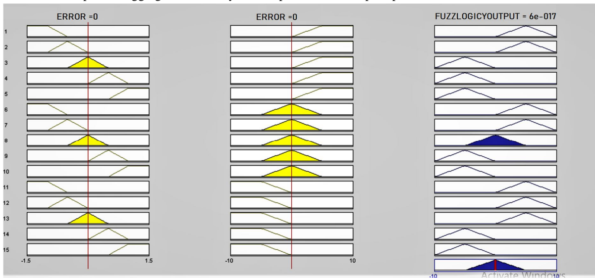
Figure 7a: Fuzzy Output Response Aggregate for "NO CHANGE"
