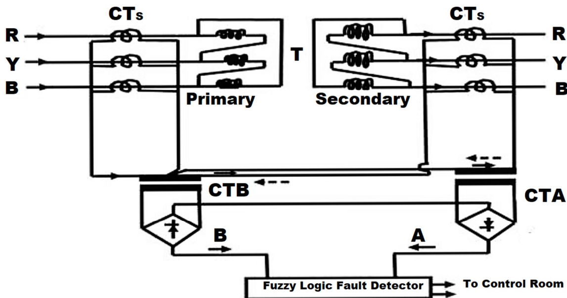
Figure 2: Improve Circuit For Detection using fuzzy logic
