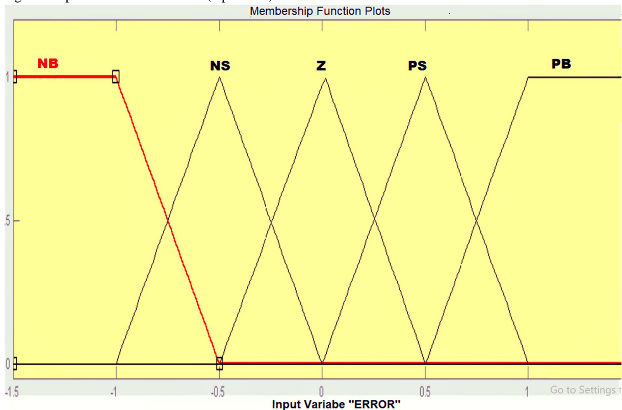
Figure 4: Error Membership Function.
