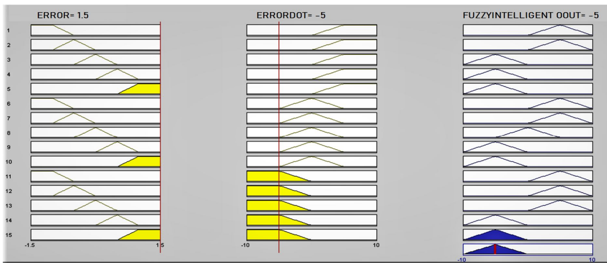
Figure 7c: Fuzzy Output Response Aggregate for "Low Current"
