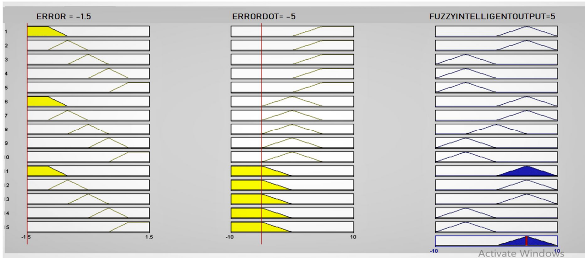
Figure 7b: Fuzzy Output Response Aggregate for "High Current"
