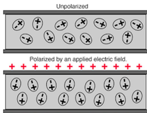
Fig. 1. Electric polarization
