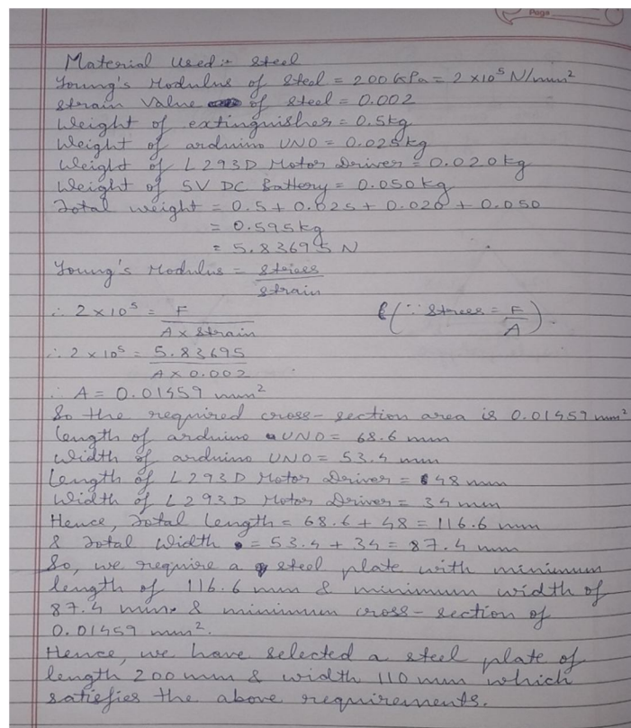
Fig. 6: Calculations for Robot
