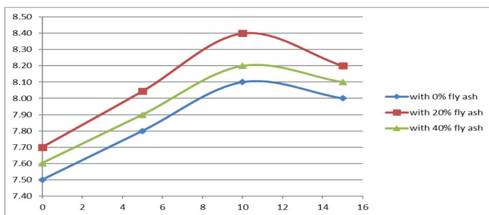
Fig. 6: Variation of flexural strength with various percentages of Fly ash and Silica Fume with 1% fibre
