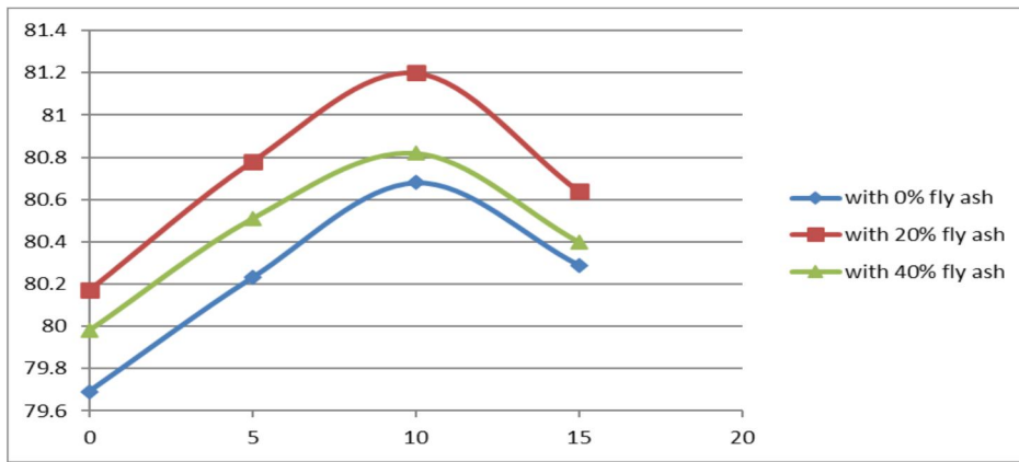
Fig. 3: Variation of compressive strength with various percentages of Fly ash and Silica Fume with 1% fibre
