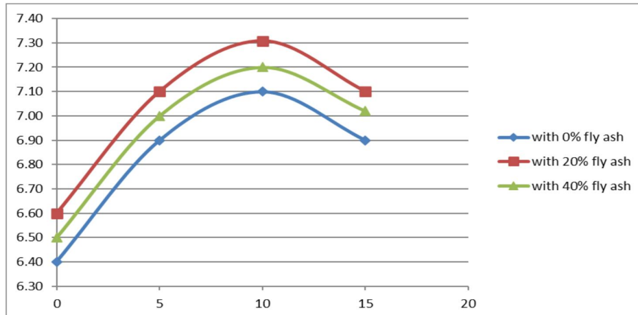
Fig. 4: Variation of flexural strength with various percentages of Fly ash and Silica Fume with 0% fibre
