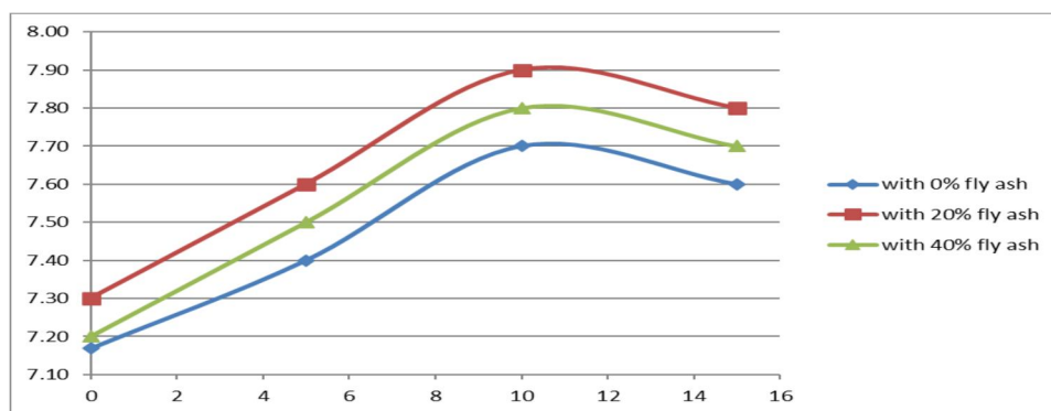
Fig. 5: Variation of flexural strength with various percentages of Fly ash and Silica Fume with 0.5% fibre
