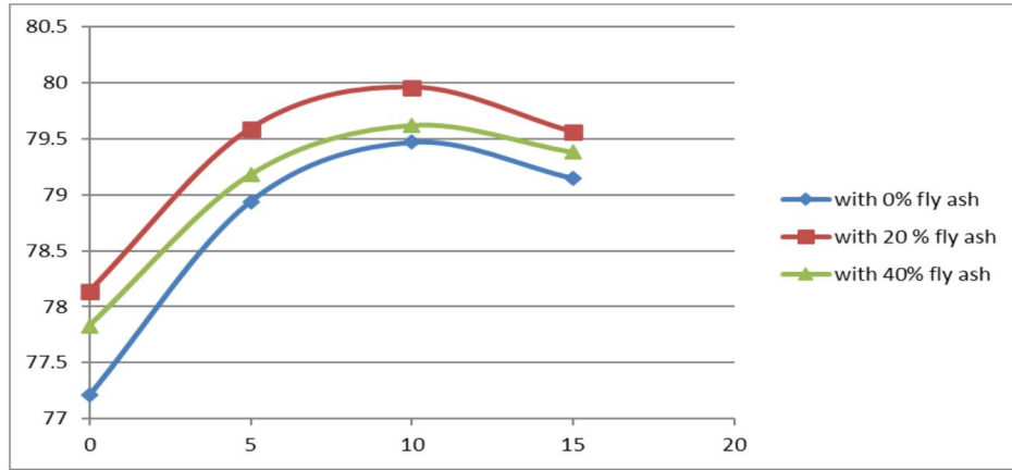
Fig. 2: Variation of compressive strength with various percentages of Fly ash and Silica Fume with 0.5% fibre
