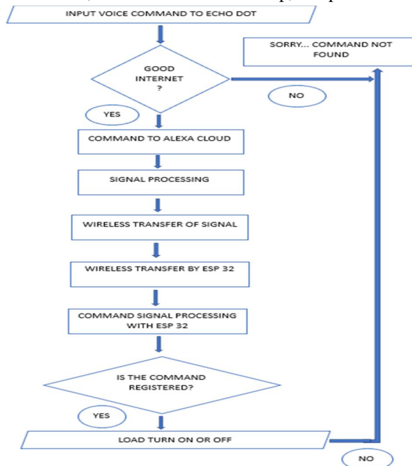
Fig.2 System Flowchart
