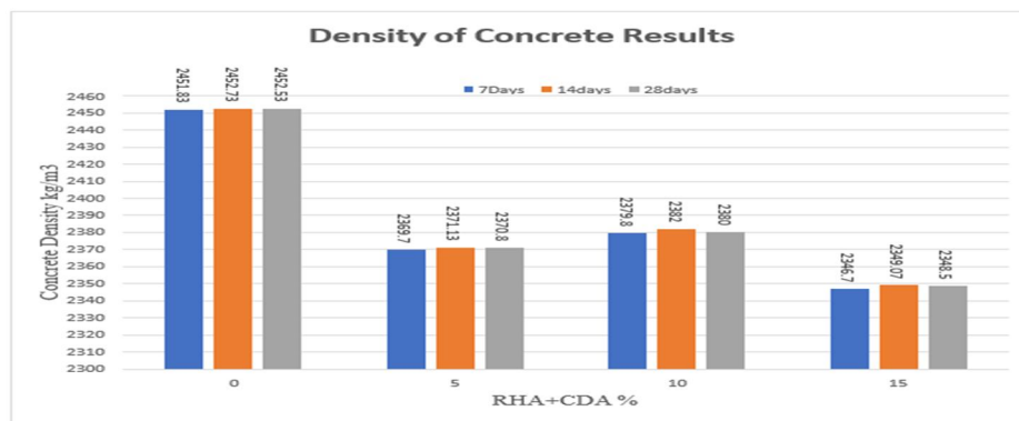
Fig. 7: Density results for various RHA+CDA% mix at 7,14,28 days curing
