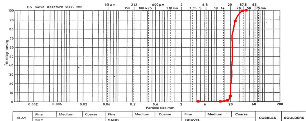
Fig. 5: Gradation Curve for Coarse Aggregate
