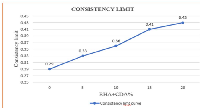
Fig. 3: Consistency curve for RHA+CDA concrete mix
