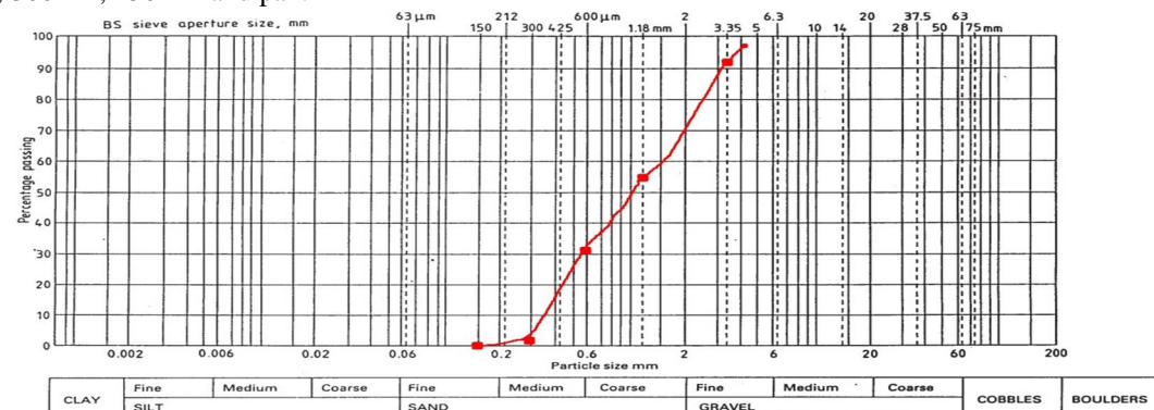
Fig. 4: Gradation Curve for Fine Aggregate
