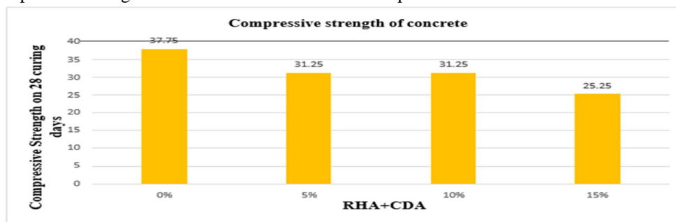
Fig. 8: Compressive strength results for various RHA+CDA% mix at 28 days curing
