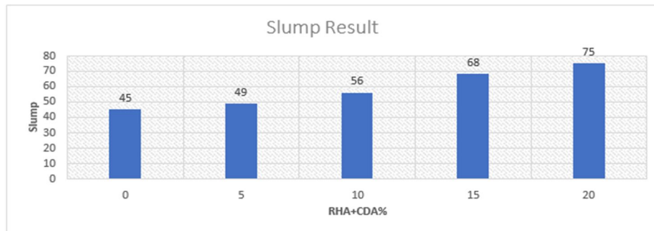
Fig. 6: Slump values for various RHA+CDA% mix
