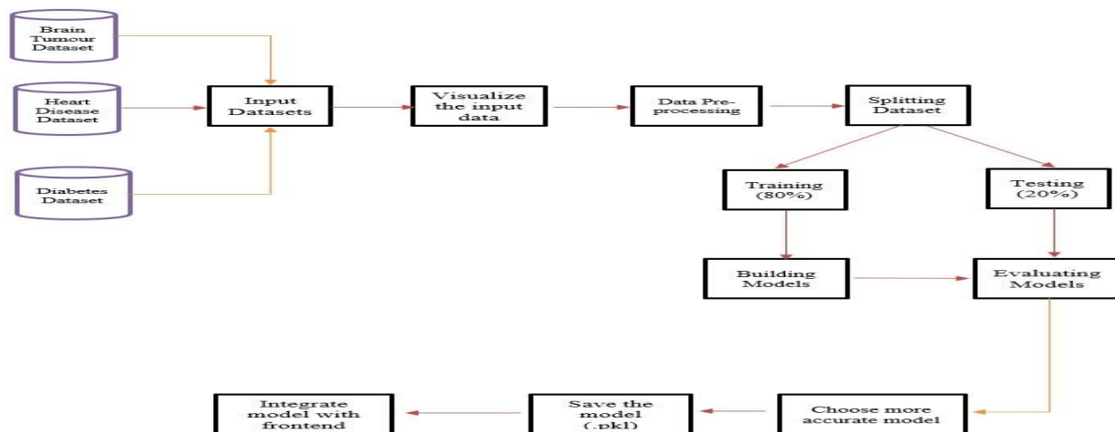
Fig. 1 System Architecture
